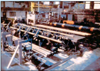
Rods and pipes handling, after.
